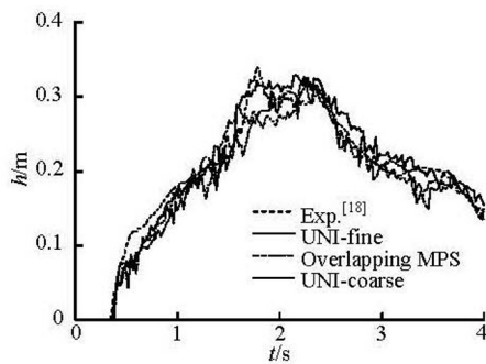
Fig.5 Time histories of water heights
