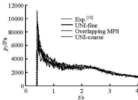
Fig.6 Impact pressure time histories at probe P_1
