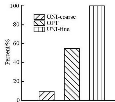
Fig.7 Comparison of required CPU time for flowing 4 s
