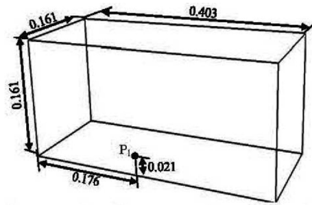
Fig.3 Locations of pressure probes on the box (m)
