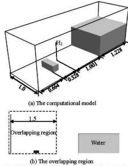
Fig.2 Geometry of the dam break (m)
